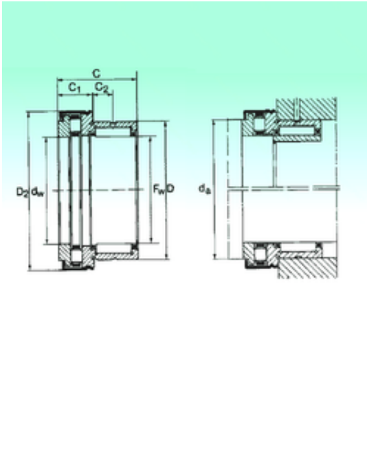
NKXR 35 Z Bearing 2D drawings and 3D CAD models
